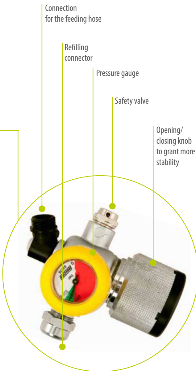
Brass alloy nickel plated pressure reducer
